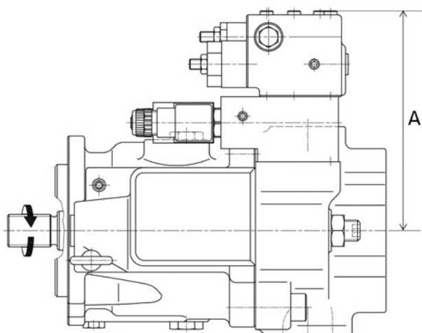
Unloading valve module (Type N,M)
