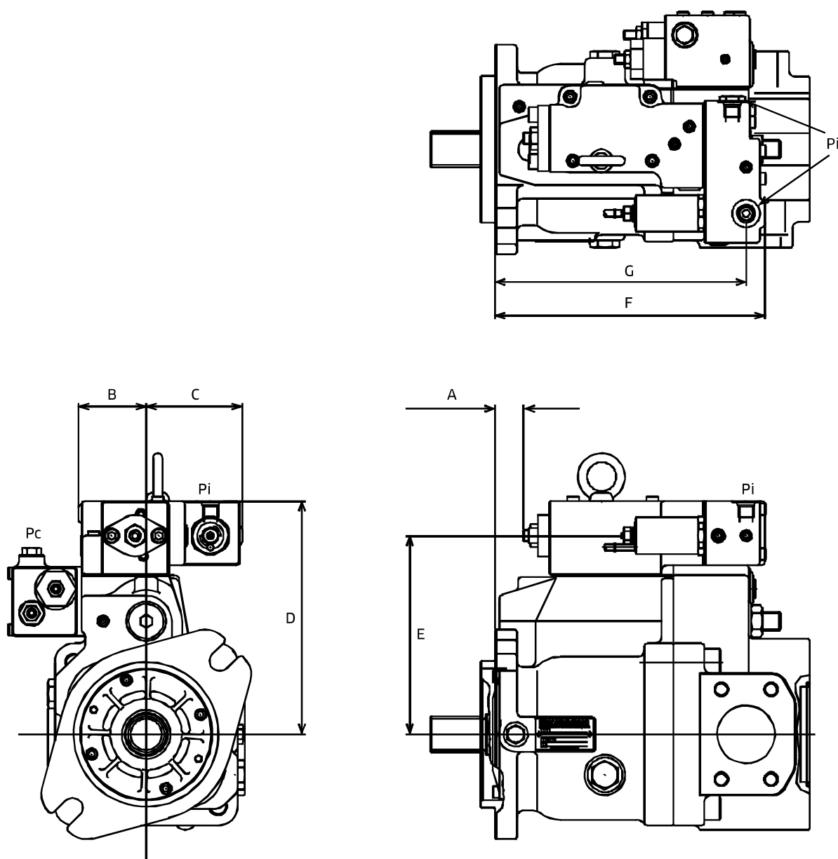
Installation Dimensions (mm)
