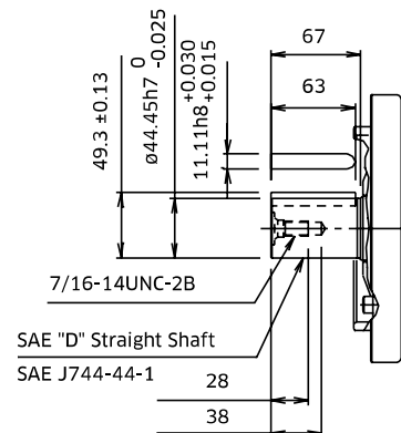
SAE 'D' Straight Shaft
