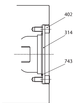
COVER Kit
