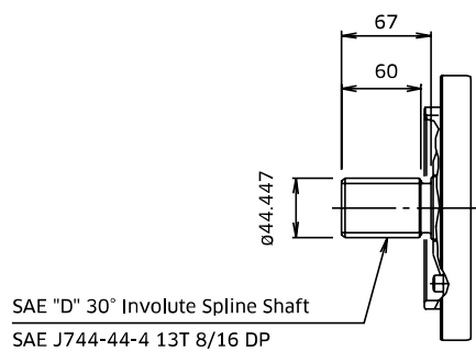
SAE 'D' Spline Shaft
