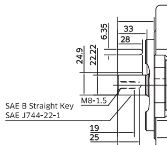
Model Code Option 'K' Shaft
