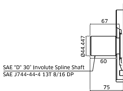
SAE Spline 'D' Shaft
