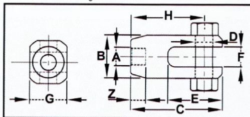
CEB XX-Base
