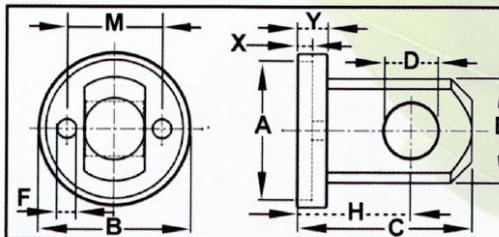
CEB XX-Base
